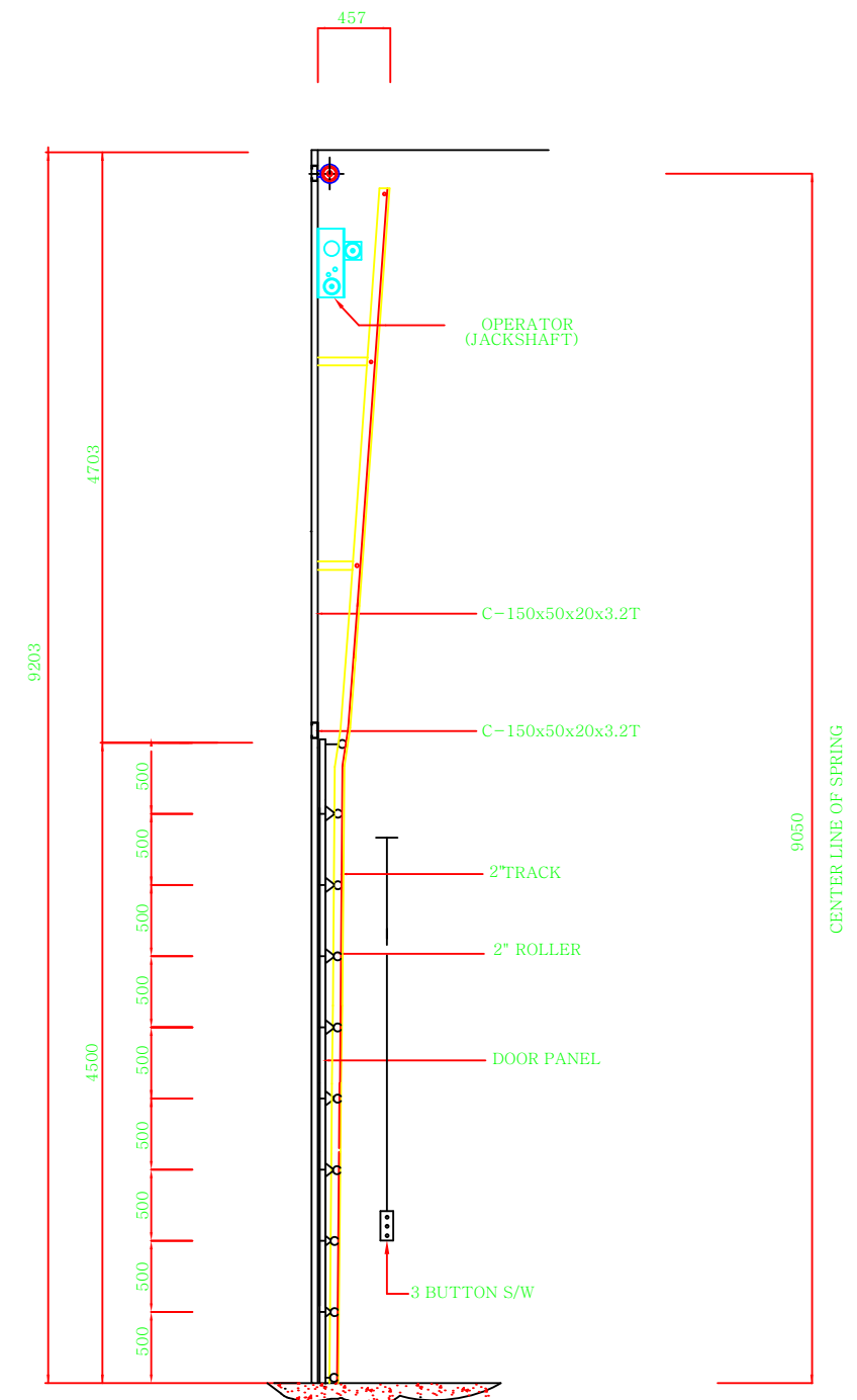
① VERTICAL LIFT SCALE 1/50
